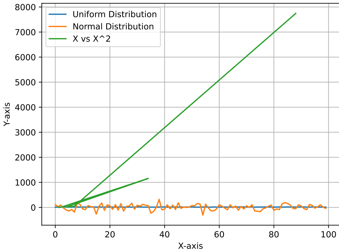
Uniform vs Normal Distribution
